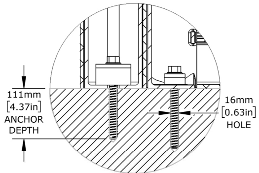
Fixing Detail
