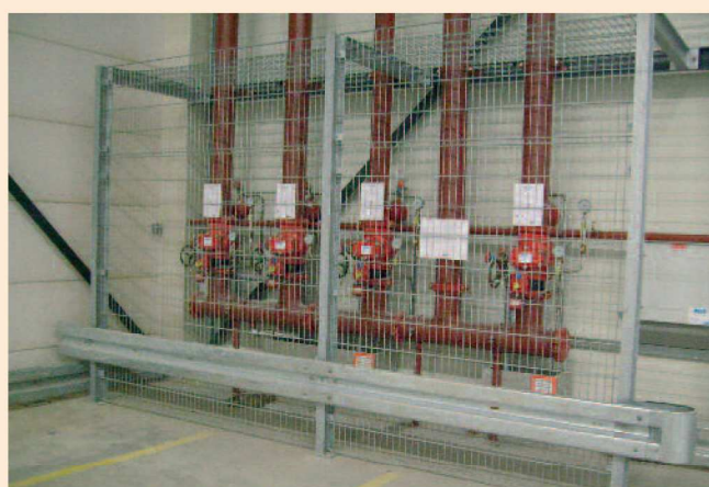
Vangrail B-profiel
