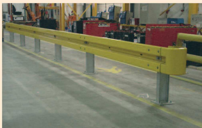
Vangrail B-profiel
